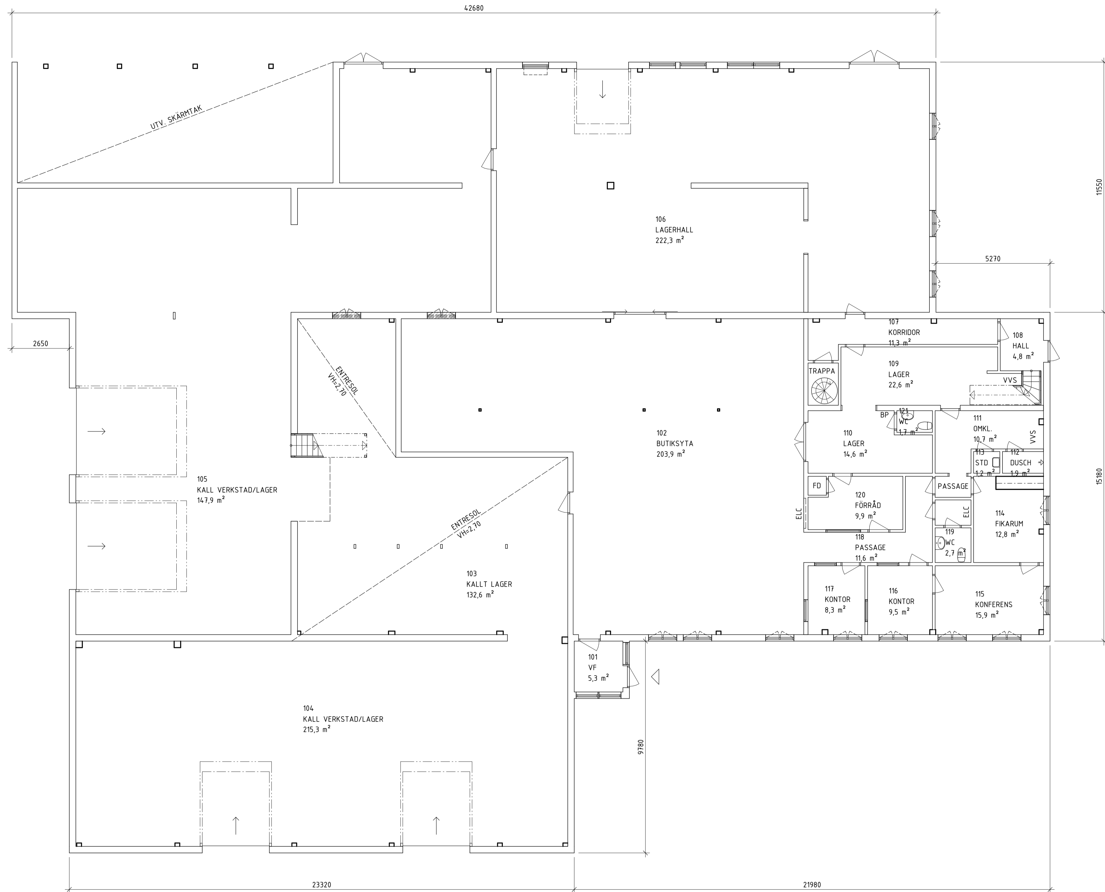
PLAN 1 1 : 100 LOA: CA. 1277m 2
