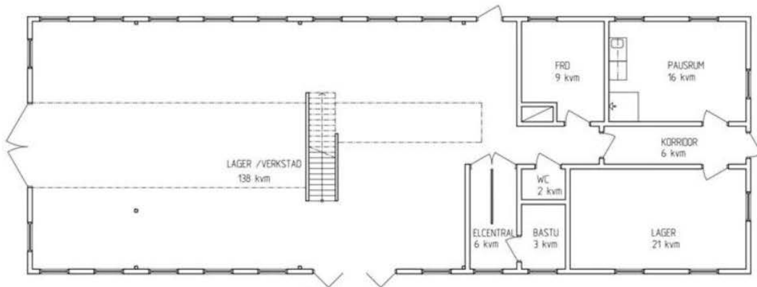
PLAN 1, BOTTENPLAN 206m 2
