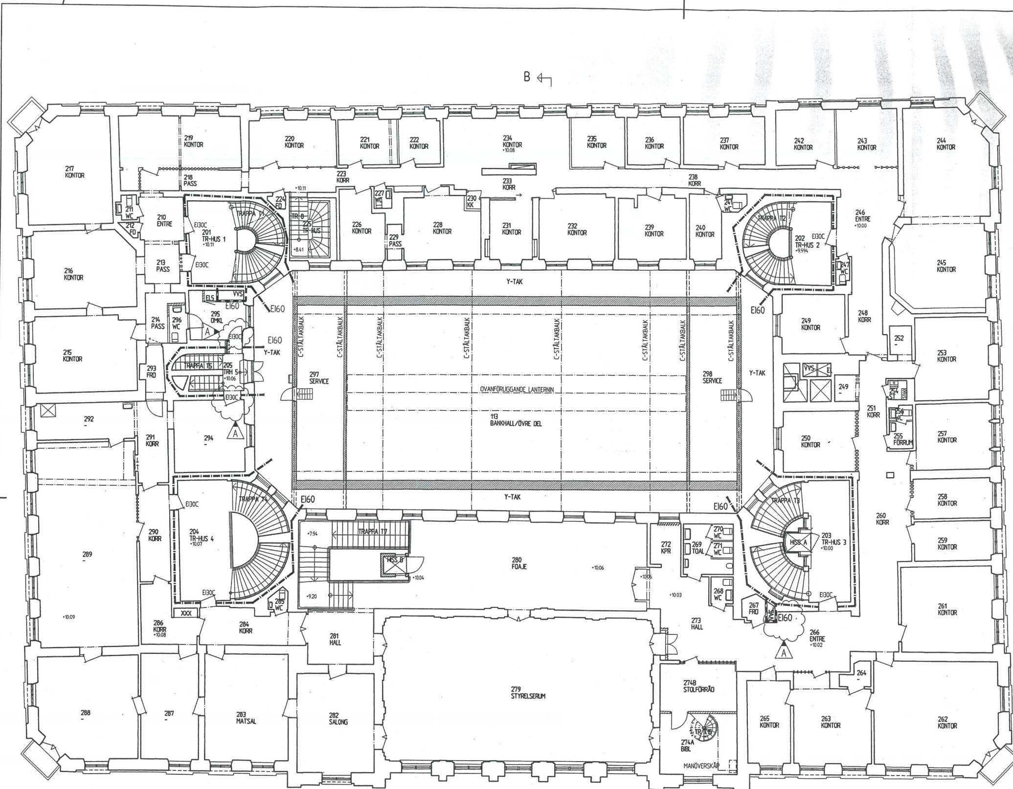
ENTRESOL PLAN 2.5
