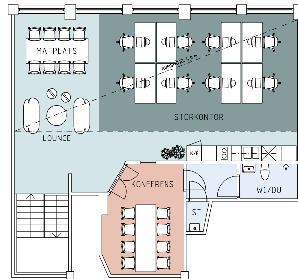
PLAN 1 TR
