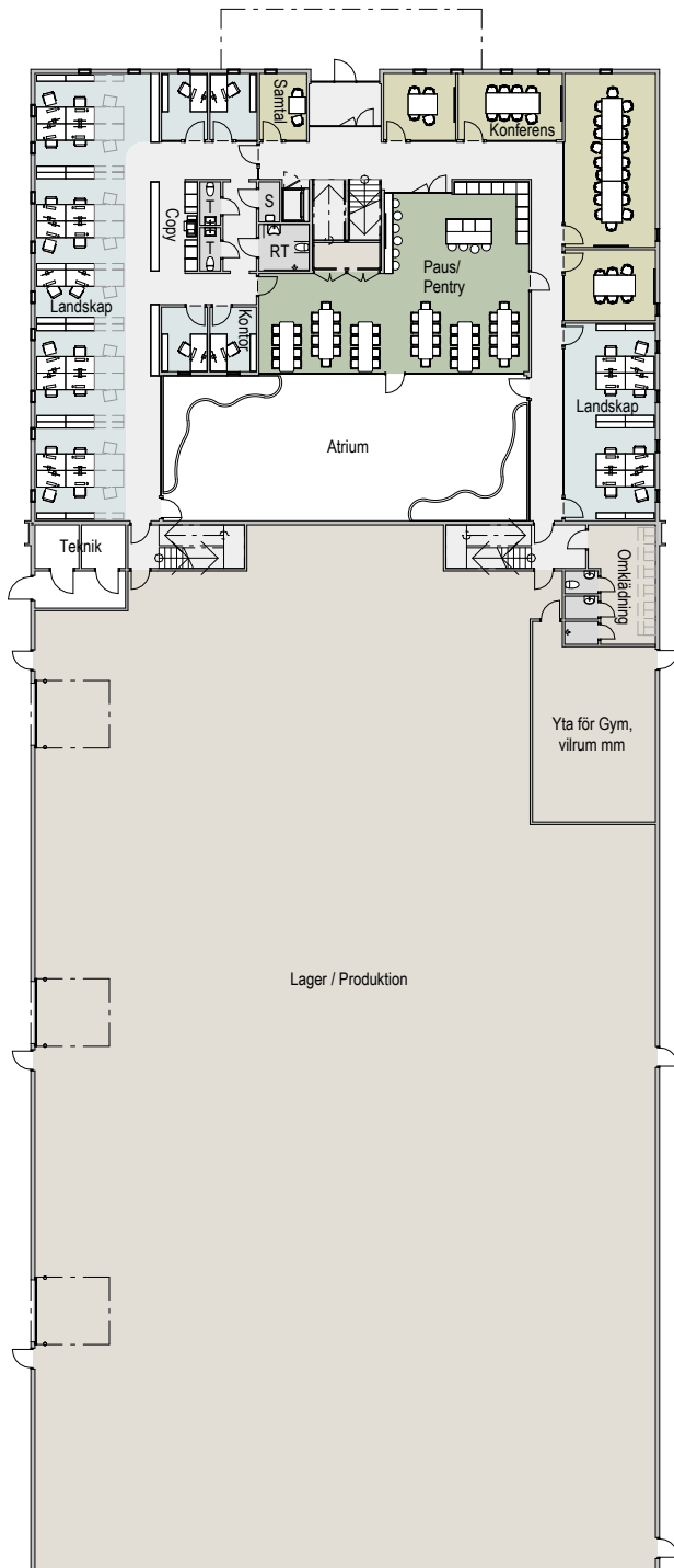
Bottenplan
